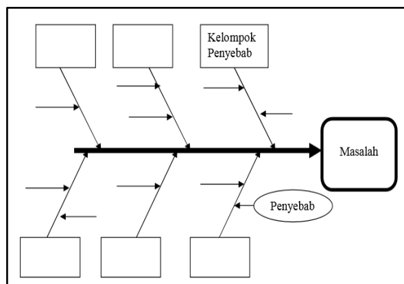
Gambar 2. Diagram Fishbone
